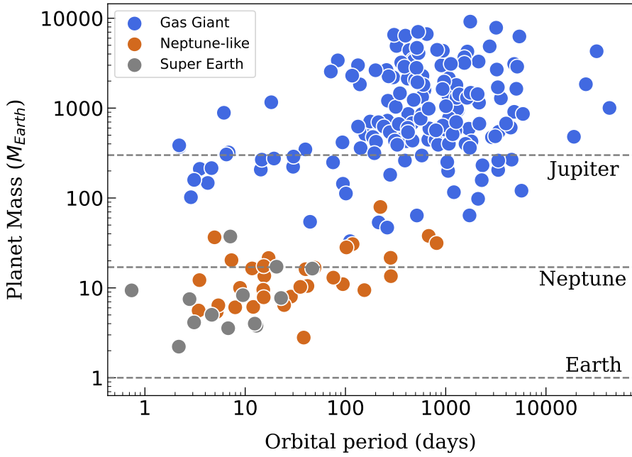
Figure 10: Planetary mass plotted against orbital period for all confirmed planets in the sample. Data points are colour-coded by planet type (super-Earths, Neptune-like, and gas giants). Reference lines corresponding to the masses of Earth, Neptune, and Jupiter are shown for comparison.
