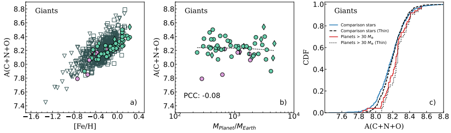
Figure 15: In panel a : Distribution of A(\text{C+N+O}) abundances with respect to [\text{Fe/H}] . Panel b : Same abundances versus planet mass for giant stars. Panel c : Cumulative A(\text{C+N+O}) distributions for giant stars. All symbols in panel (c) have the same meaning as in Fig 14.
