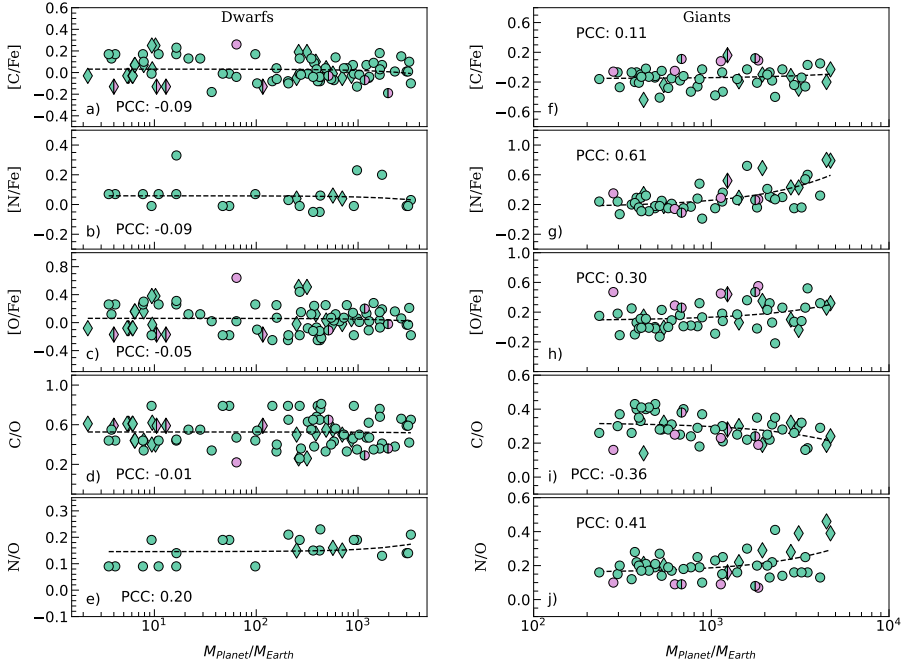
Figure 23: [\text{C}/\text{Fe}] , [\text{N}/\text{Fe}] , [\text{O}/\text{Fe}] abundances and \text{C}/\text{O} , \text{N}/\text{O} ratios as functions of planet masses for investigated dwarfs (left panel) and giants (right panel). All planets in multi-planet systems are considered in this figure. All symbols have the same meaning as in Fig. 22.
