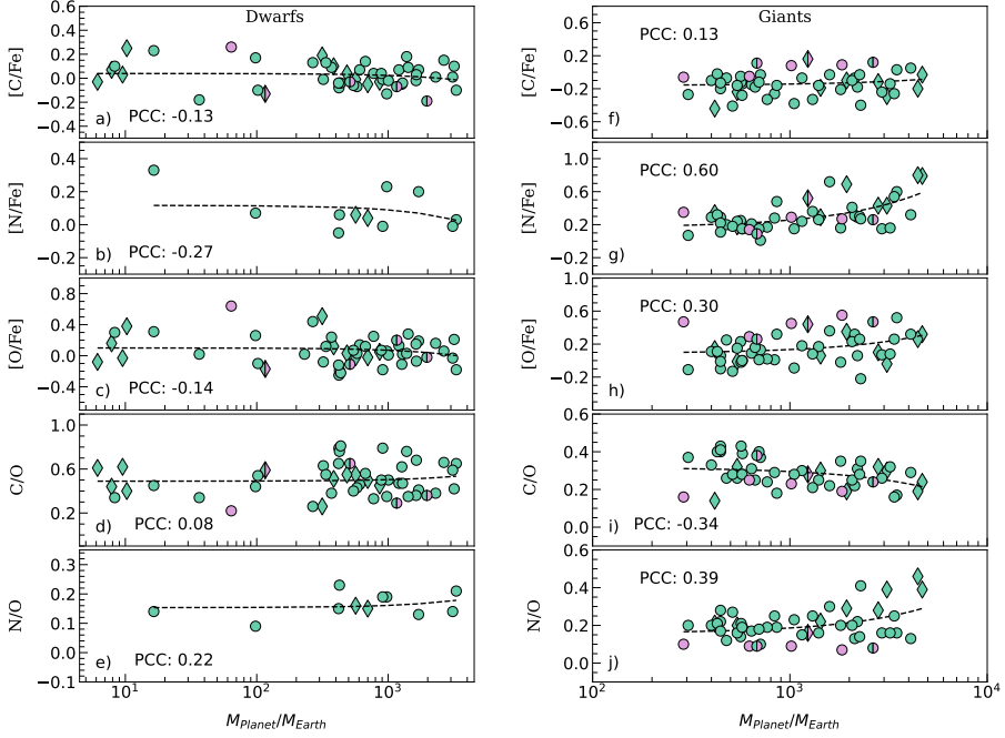
Figure 22: [\text{C}/\text{Fe}] , [\text{N}/\text{Fe}] , [\text{O}/\text{Fe}] abundances and \text{C}/\text{O} , \text{N}/\text{O} ratios plotted as functions of planet masses for investigated dwarfs (left panel) and giants (right panel). For multi-planet systems, only the most massive planet is considered. Green circles and diamonds represent thin disc stars, while pink circles represent thick disc stars. Linear regression fits were added as dashed lines.
