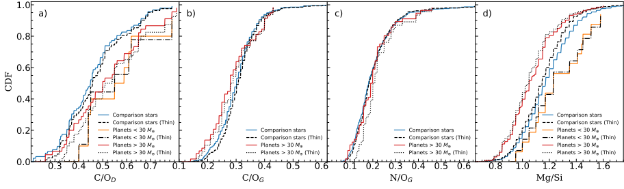
Figure 14: Cumulative distribution functions (CDFs) of elemental ratios C/O, N/O, and Mg/Si for stars with and without detected planets. Panel a : shows the cumulative C/O distributions for dwarfs. Solid orange and red lines represent hosts of low-mass ( M_p < 30M_{\oplus} ) and high-mass ( M_p > 30M_{\oplus} ) planets, respectively, while the solid blue line corresponds to comparison stars without planets. Black lines denote the corresponding thin-disc subsamples. Panels b and c : display the cumulative distributions of C/O and N/O ratios for giant stars, and panel d : shows the cumulative Mg/Si distributions for all stars with planetary companions compared to the control sample.
