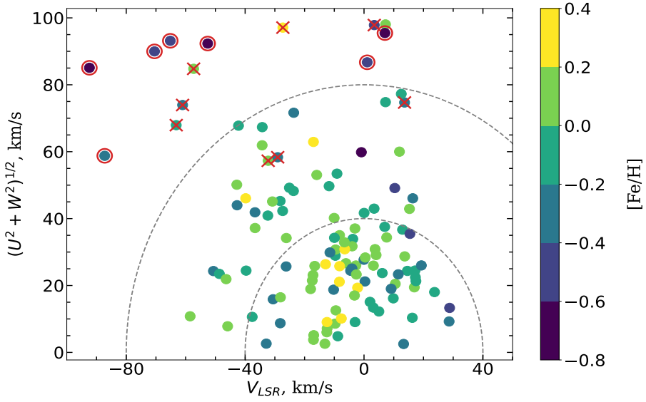
Figure 7: Toomre diagram for the analysed stars, with symbols colour-coded by metallicity [\text{Fe}/\text{H}] . The diagram displays the combined transverse velocity, (U^2 + W^2)^{1/2} , plotted against the rotational velocity relative to the Local Standard of Rest, V_{\text{LSR}} . Dashed curves represent contours of constant total space velocity ( v_{\text{tot}} = (U_{\text{LSR}}^2 + V_{\text{LSR}}^2 + W_{\text{LSR}}^2)^{1/2} ) at 40 and 80 \text{km s}^{-1} . Stars outlined in red correspond to thick-disc members, while crosses mark intermediate thin/thick-disc stars.
