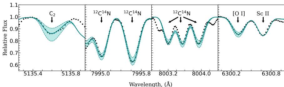
Figure 2: Example of spectral synthesis for representative molecular and atomic features used in the abundance analysis. Observed spectra are shown as black dots, while the solid green line represents the best-fitting synthetic spectrum, with dashed lines indicating variations of \pm 0.10 dex from the optimal abundance.
