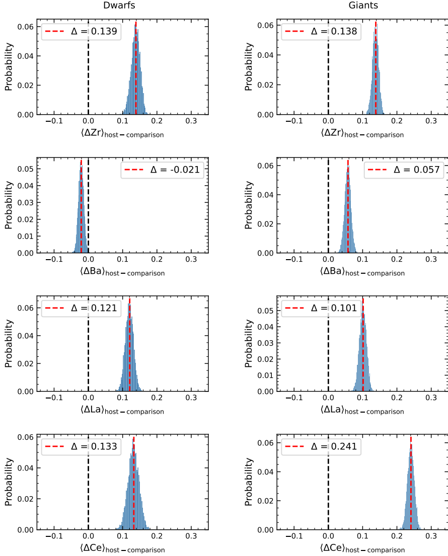
Figure 18: Bootstrap distributions of mean abundance differences ( \Delta = [\text{X}/\text{Fe}]_{\text{host}} - [\text{X}/\text{Fe}]_{\text{comparison}} ) for selected n -capture elements (Zr, Ba, La, and Ce) in dwarfs and giants. Each histogram represents the result of 10 000 re-sampled comparisons with a control sample matched in T_{\text{eff}} , \log g , and [\text{Fe}/\text{H}] . Vertical dashed lines mark \Delta = 0 (black) and the observed mean \Delta (red). Histograms are normalized to show probability per bin.
