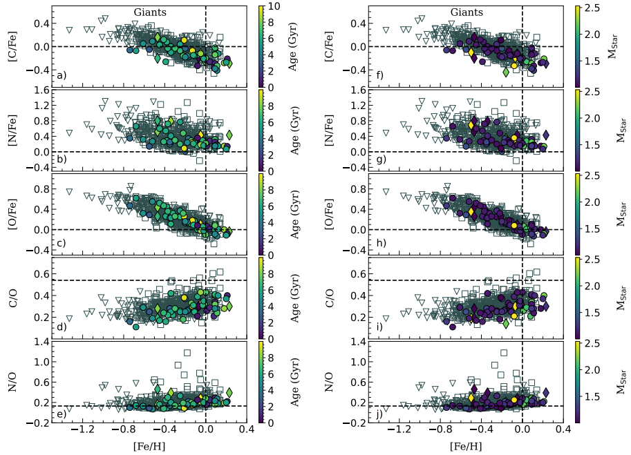
Figure 12: [X/Fe] abundance ratios for carbon, nitrogen, and oxygen, together with derived C/O and N/O ratios as functions of metallicity [Fe/H] for observed giant stars. The left-hand panel shows stars colour-coded by stellar age, and the right-hand panel by stellar mass. All symbol shapes have the same meaning as in Fig. 11.
