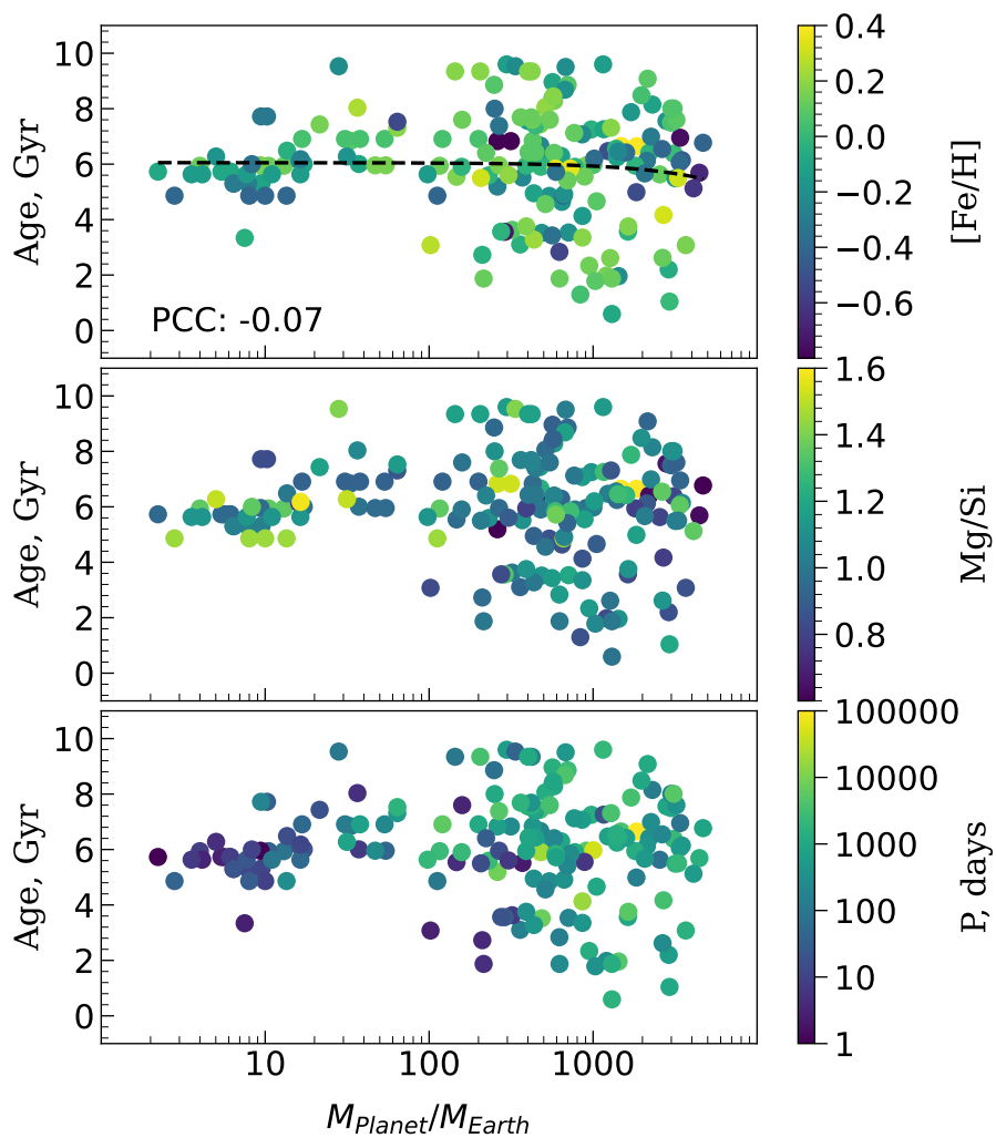
Figure 27: Distribution of stellar age versus planet mass colour-coded by [\text{Fe}/\text{H}] (top panel), \text{Mg}/\text{Si} (middle panel) & orbital period of the planets (bottom panel). Refer to the text for more information.
