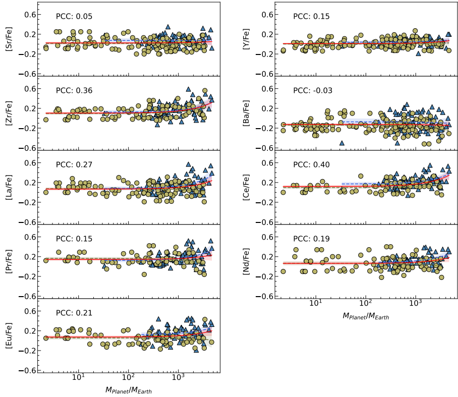
Figure 26: Abundances of neutron-capture elements [El/Fe] shown as functions of planet masses for all investigated planetary systems. All symbols have the same meaning as in Fig. 17. Refer to the text for more information.
