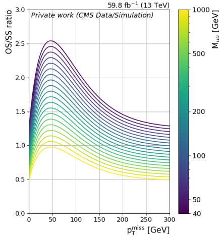
Fig. 24: One-dimensional slices of the fitted OS/SS transfer factor R_{\text{OS/SS}}(M_{\mu\mu}, p_T^{\text{miss}}) in the sideband for 2018 data.
