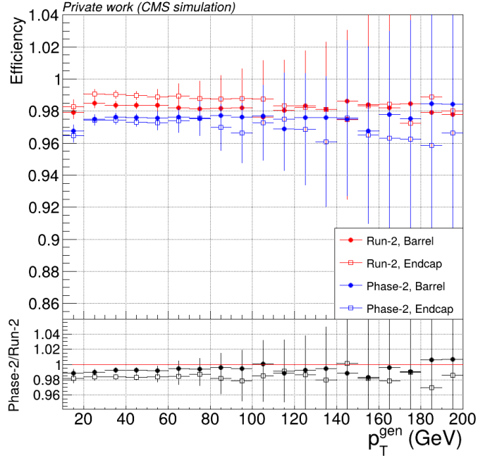
Fig. 68: Comparison of the global-muon reconstruction efficiency in Run-2 and Phase-2 as a function of the generator-level muon transverse momentum. The results are shown separately for the barrel ( |\eta| < 1.2 ) and endcap regions. The lower panel shows the ratio of the Phase-2 and Run-2 efficiencies.
