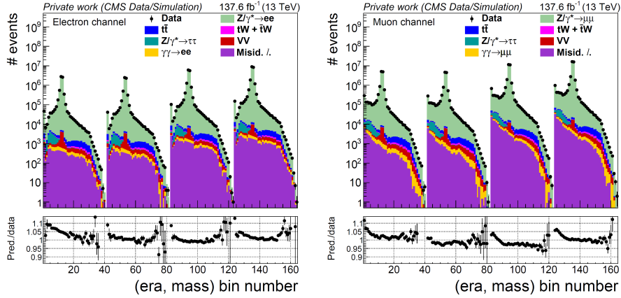
Fig. 41: Reconstructed invariant mass distributions for electrons (left) and muons (right), split by data-taking era. Each Z boson peak corresponds to a different era.
