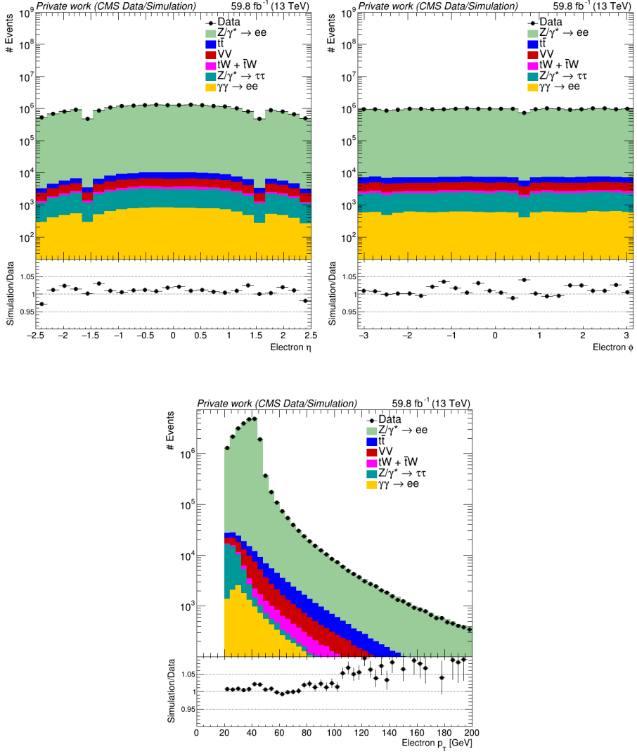
Fig. 20: Subleading-electron kinematic distributions for 2018 data and simulation after event selection and corrections.
