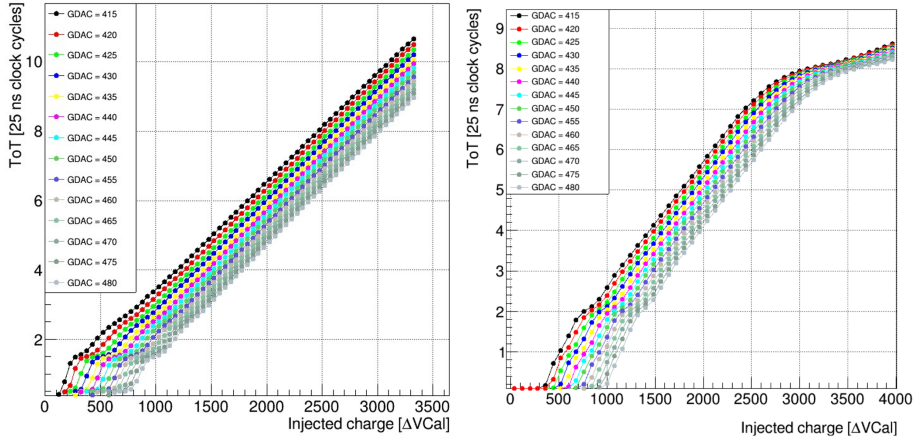
Fig. 62: Average ToT response as a function of injected charge for different hit-detection threshold settings. Left: without 6-to-4-bit compression; right: with 6-to-4-bit compression enabled. The Krummenacher current is fixed to 100 DAC units.
