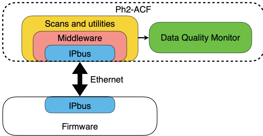
Fig. 54: Ph2-ACF software architecture [24].
