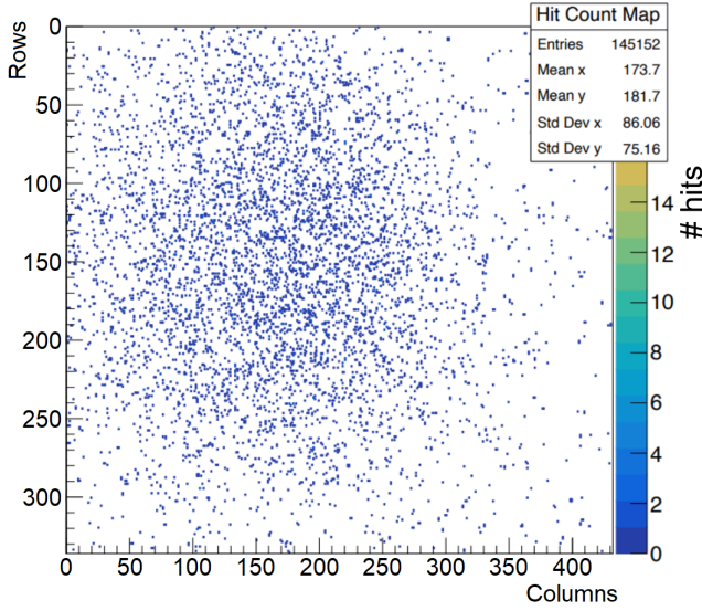
Fig. 66: Hit map of the recorded ^{241}\text{Am} X-ray events on the pixel matrix.
