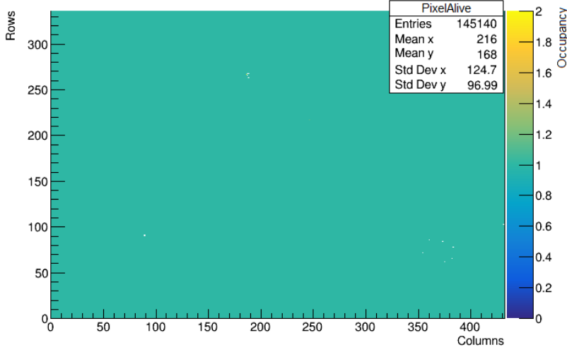
Fig. 55: Example of a two-dimensional pixel occupancy map produced by the PixelAlive scan.
