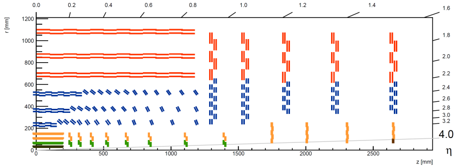
Fig. 50: A one-quarter slice of the CMS Phase-2 Tracker in the r - z plane [137]. The red and blue lines show modules of the Outer Tracker, while the yellow, orange, green, and brown lines denote modules of the Inner Tracker.
