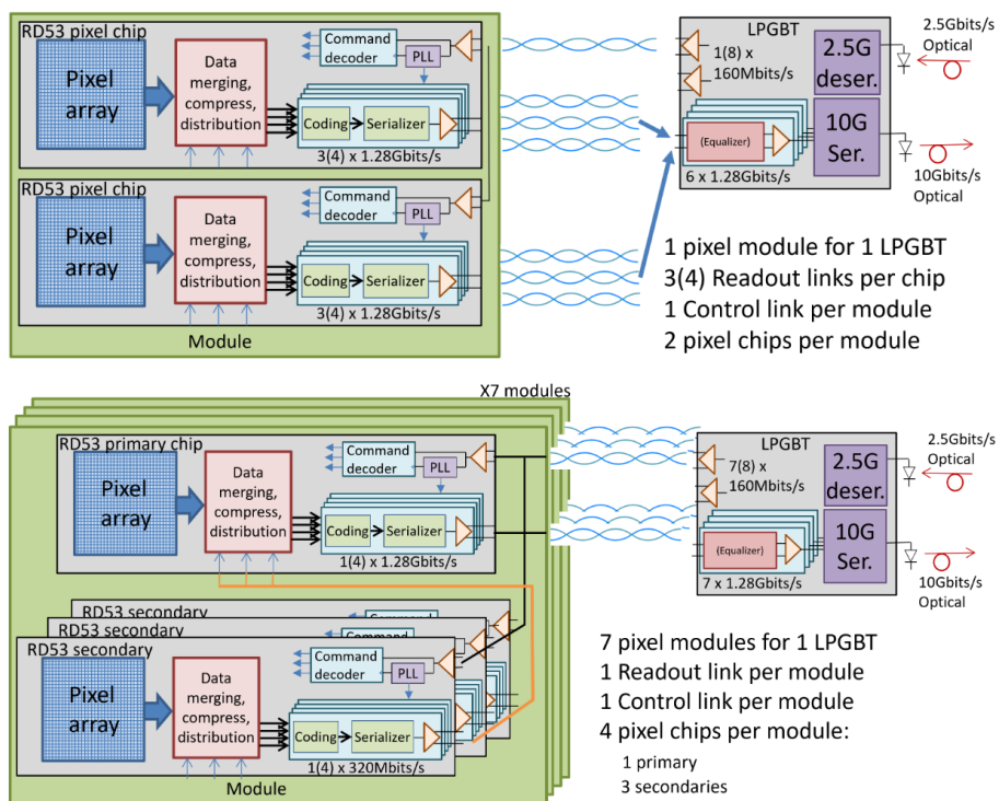
Fig. 51: The IT module readout chain using e-links. Top: Inner Barrel layer module with two pixel chips connected to one lpGBT. Bottom: outer IT layer module with four pixel chips per module and local data aggregation. Adapted from Ref. [137].
