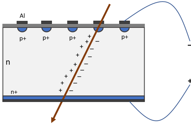
Fig. 15: A sketch of a p-in-n silicon sensor operation. A charged particle traversing the sensor creates electron-hole pairs, which are separated by the electric field and collected by the electrodes. Reversing the doping types and voltage polarity gives the corresponding n-in-p or n^+ -in-n sensor configurations.
