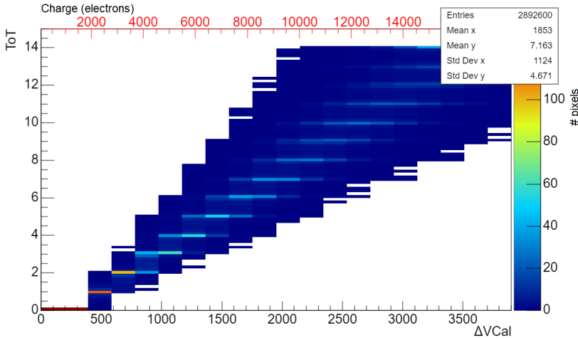
Fig. 57: Example of superimposed gain curves for all pixels on a chip, produced by the Gain scan without ToT compression.
