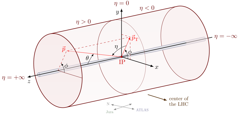
Fig. 14: The coordinate system used by the CMS detector [108].
