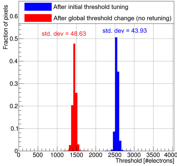
Fig. 61: Threshold distribution before (blue) and after (red) changing the global threshold while keeping the TDAC values fixed [B3].
