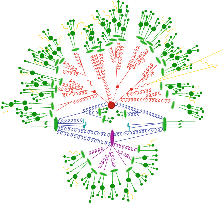
Fig. 6: A graphic representation of a proton-proton collision event as produced by an MC generator. Two large green ellipses, with three green arrows entering each, represent the colliding protons. Partons from the colliding protons are shown as blue lines, two of which meet at a large red circle representing the hard interaction. The red lines represent particles produced in the hard interaction, some of which decay promptly, as indicated by the small red circles. The outgoing colored partons then undergo hadronization, shown by the light-green ellipses, and unstable hadrons decay into longer-lived particles, represented by smaller dark-green circles. The purple ellipse represents the underlying event, while the light-blue ellipses show the proton remnants. Photon radiation, shown as yellow lines, may occur at different stages of the event [47].
