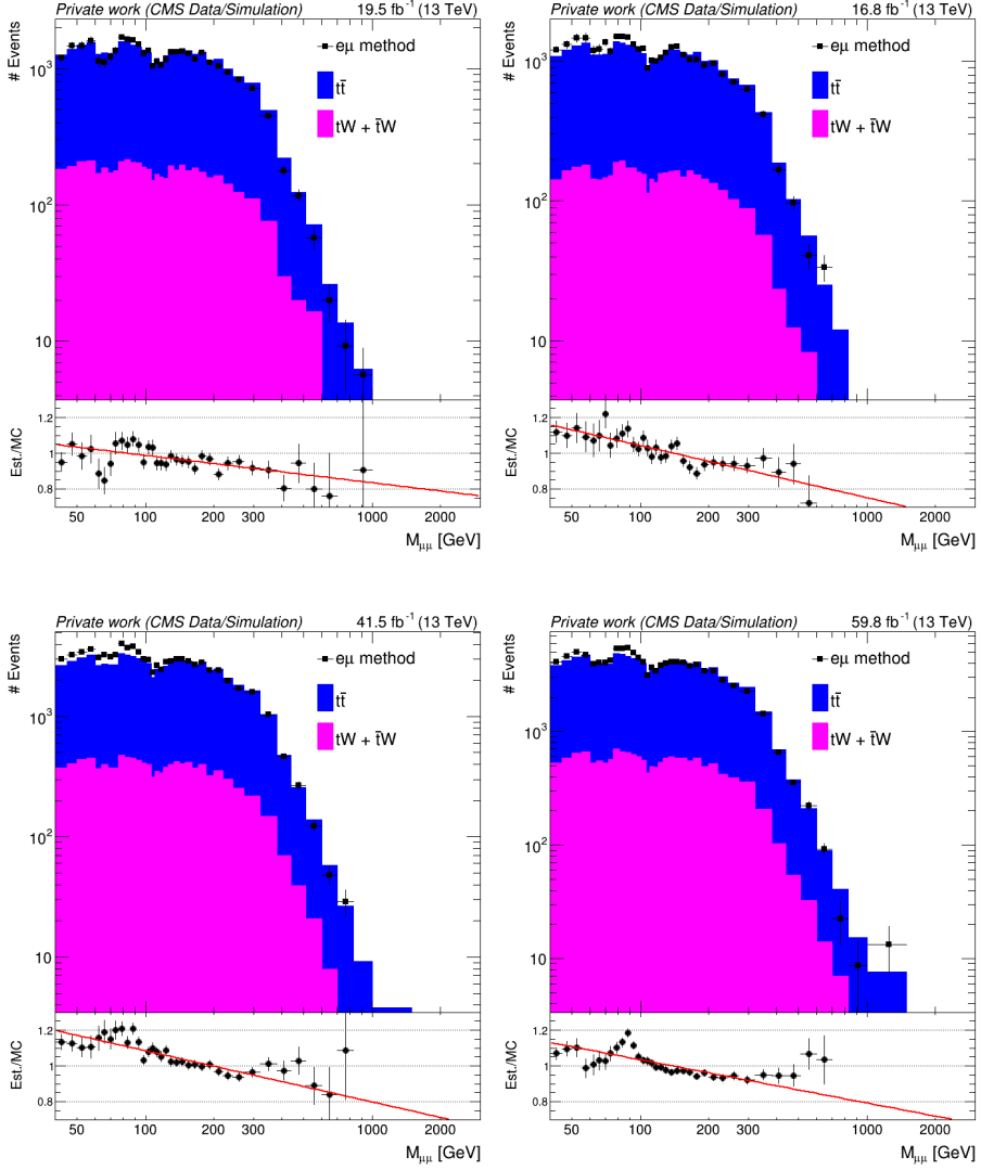
Fig. 31: Ratio of the modified e\mu method prediction to the nominal simulated top-quark background in the dimuon channel for each era. The red line shows the linear fit in \log_{10}(M_{\mu\mu}) used to define the event weight in Eq. (10.9).
