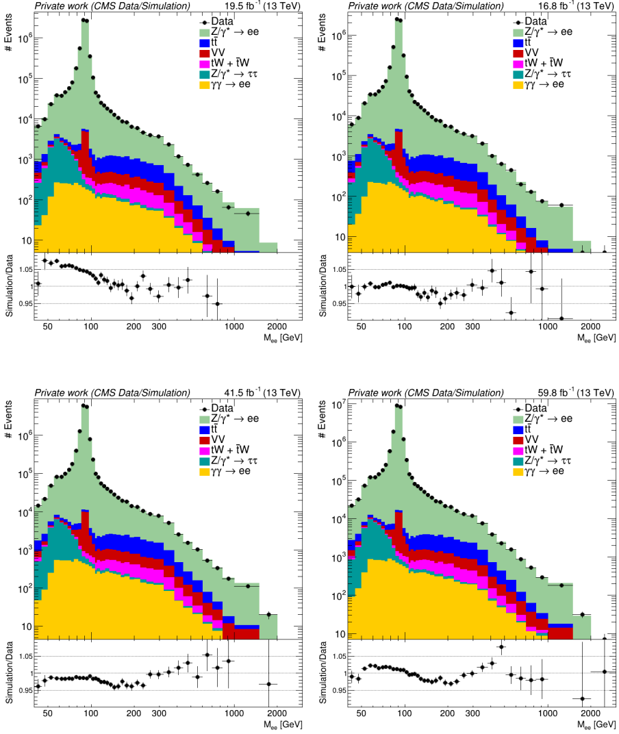
Fig. 21: Dielectron invariant mass distributions for all eras after event selection and corrections.
