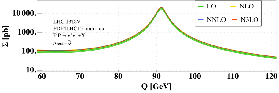
Fig. 9: A comparison of one-dimensional Drell–Yan differential cross sections \Sigma(Q^2) , Eq. (3.6) at the proton-proton collision energy \sqrt{s} = 13 TeV in the dilepton mass range 60 \leq M \leq 120 GeV, calculated at different accuracies from LO to N 3 LO in QCD [77].
