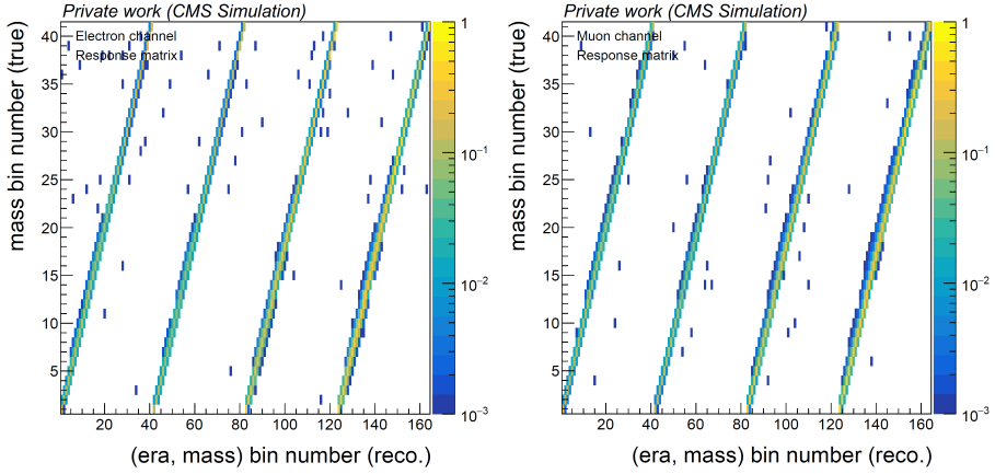
Fig. 42: Response matrices for electrons (left) and muons (right). Each diagonal block corresponds to a different data-taking era on the reconstructed axis, while the true axis corresponds to the common fiducial mass spectrum.
