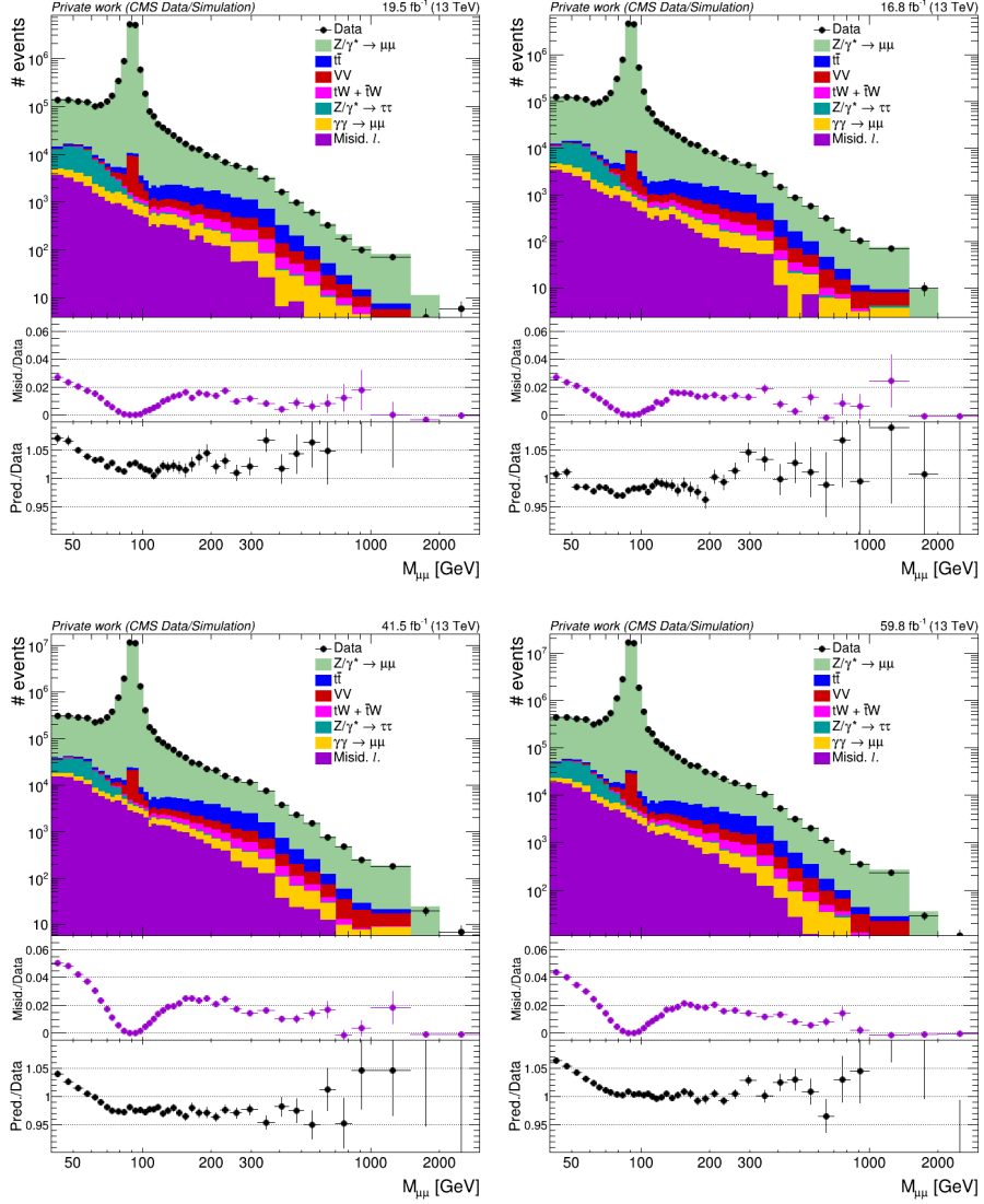
Fig. 28: Comparison between data and the sum of simulated prompt-lepton backgrounds plus the misidentified/non-prompt muon estimate in the OS dimuon signal region for each era. The middle panel shows the fraction of the observed data attributed to misidentified/non-prompt muon backgrounds, while the bottom panel shows the ratio of the total signal plus background yield prediction and the observed data.
