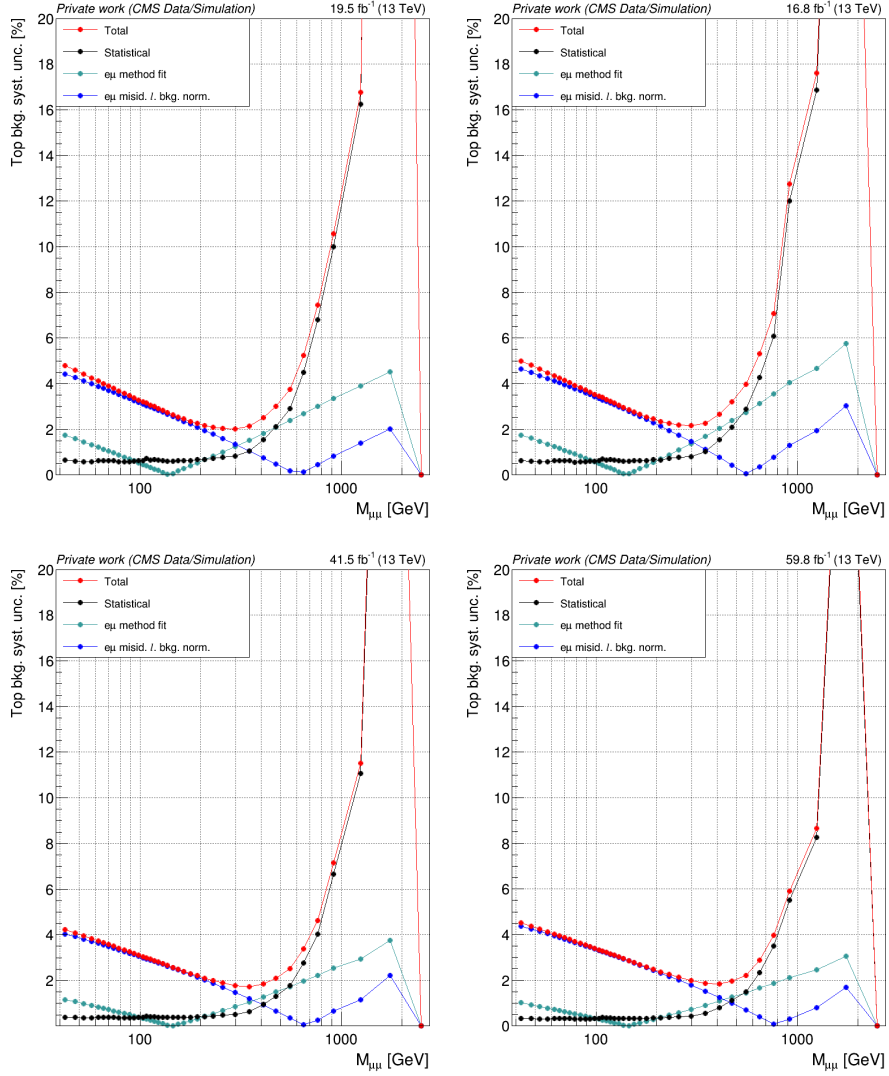
Fig. 32: Relative uncertainties on the reweighted top-quark background prediction in the dimuon channel for each era. Points with 0% uncertainty at very high mass correspond to empty bins. A single point at very high mass in each plot lies outside the vertical axis range due to limited statistics.
