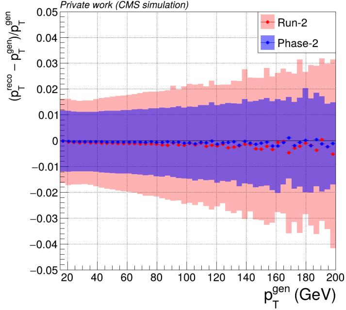
Fig. 69: Comparison of the reconstructed-to-generator response for the muon transverse momentum in Run-2 and Phase-2 as a function of the generator-level dressed muon p_T . In each generator-level bin, the response distribution is fitted with a Gaussian function. The marker points show the fitted mean, while the shaded bands indicate the fitted width \sigma , taken as the resolution.
