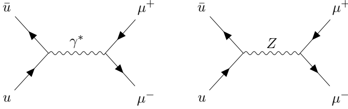
Fig. 3: Tree-level Feynman diagrams contributing to the u\bar{u} \rightarrow \mu^+\mu^- process.
