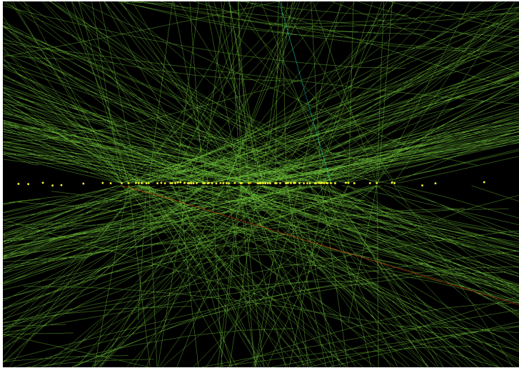
Fig. 12: An example of pileup in the CMS experiment. The image shows a collision event recorded in 2012 with multiple tracks from different interactions in the same bunch crossing. A total of 78 primary vertices were reconstructed [106].
