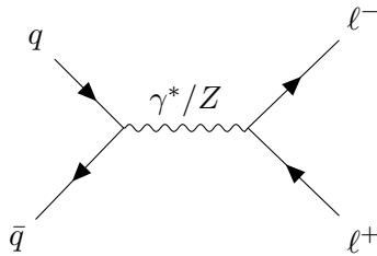
Fig. 7: Leading-order Feynman diagram for the neutral-current Drell–Yan process.
