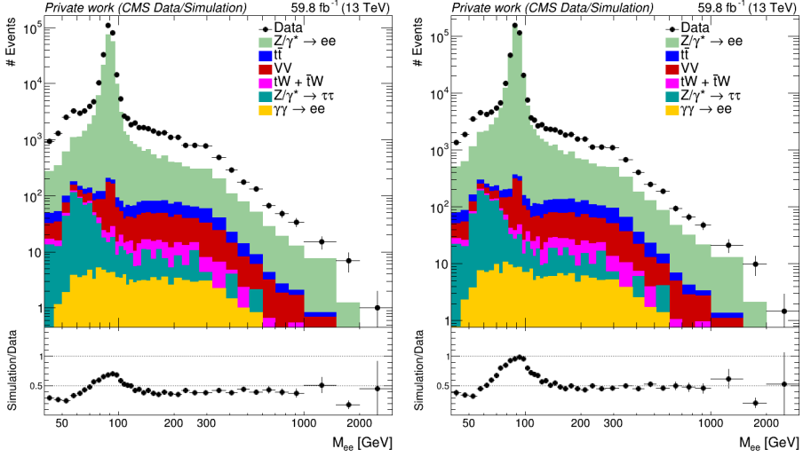
Fig. 34: Comparison between data and simulated prompt-lepton backgrounds in the SS dielectron control region before (left) and after (right) applying the charge misidentification correction, for 2018 data.
