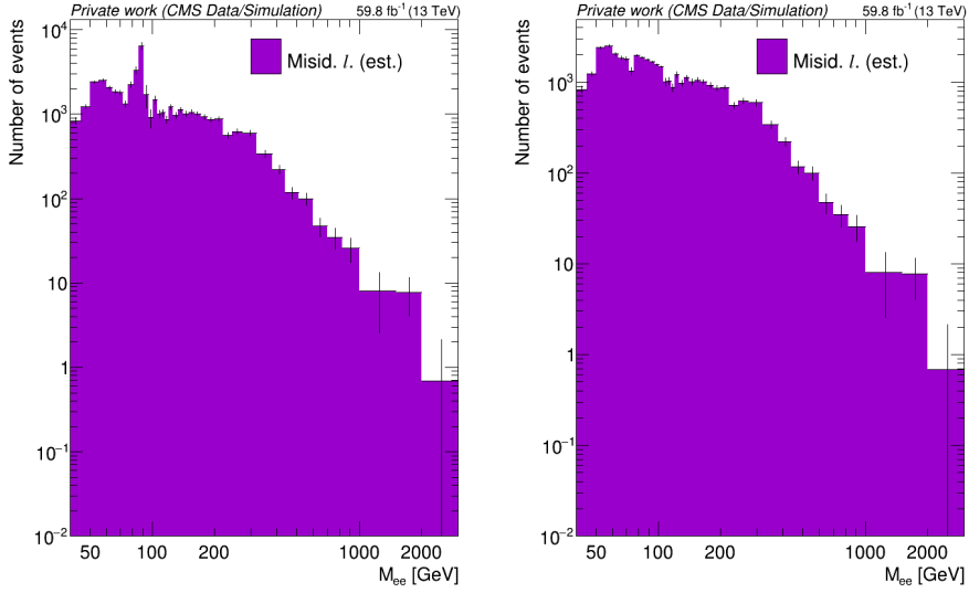
Fig. 37: Estimated misidentified/non-prompt electron background in the OS dielectron signal region for 2018 data. Left: distribution before replacing the Z -peak region; right: distribution after applying the linear interpolation.
