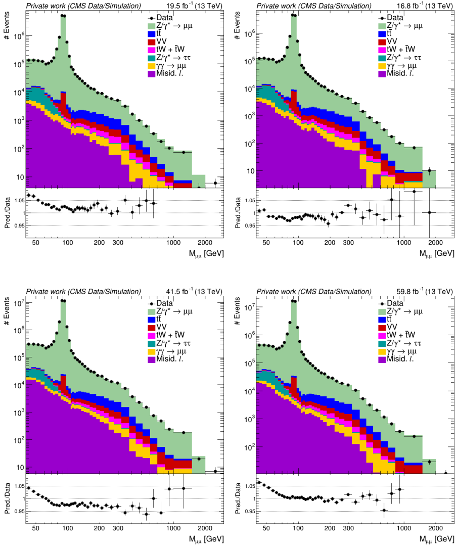
Fig. 33: Comparison between data and the total background prediction in the OS dimuon signal region, after applying the e\mu -based reweighting of top-quark backgrounds and including the misidentified/non-prompt muon estimate, for each data-taking era.
