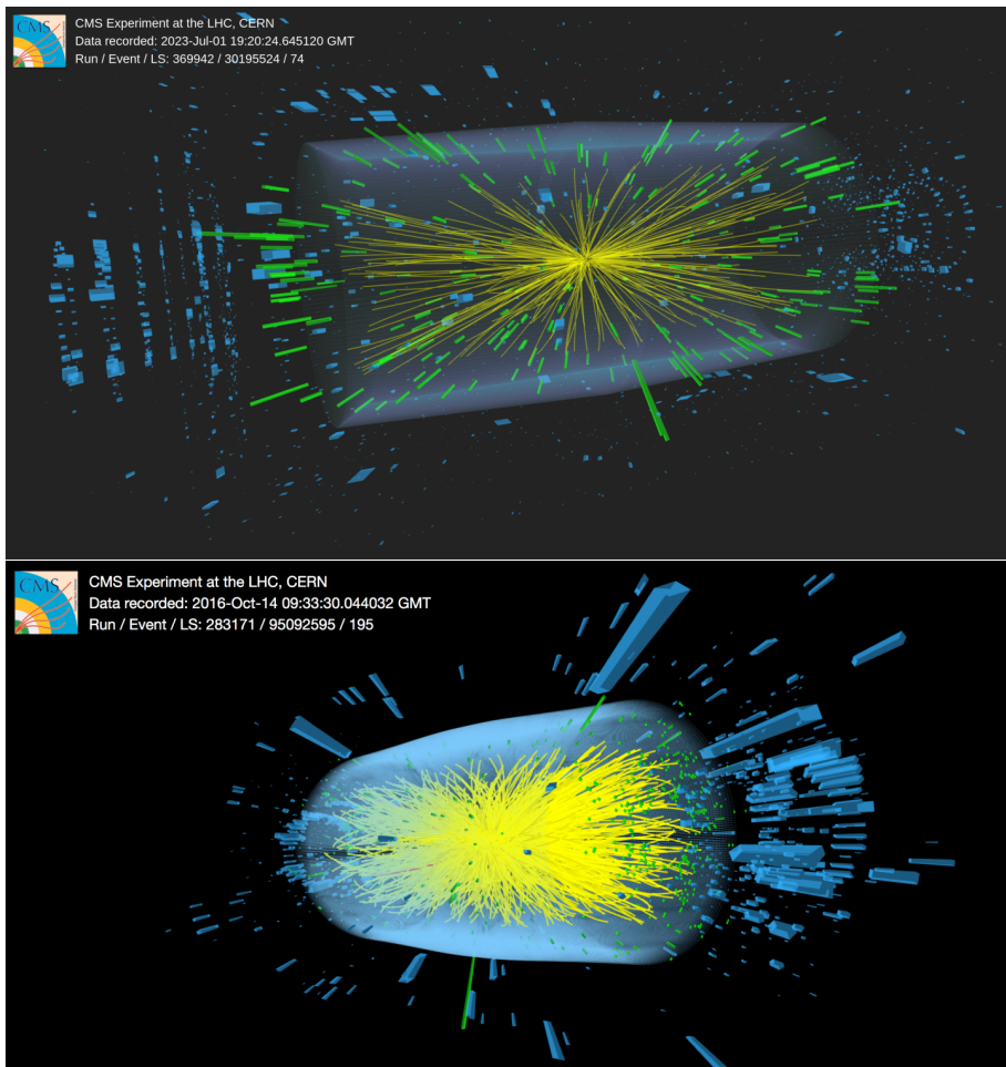
Fig. 47: Comparison of a regular-pileup event with 39 reconstructed vertices (top) [139] and a high-pileup event with approximately 100 reconstructed vertices (bottom) [140].
