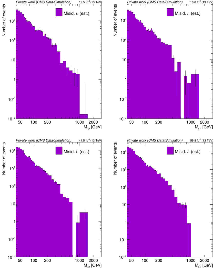
Fig. 26: Estimated distributions of misidentified/non-prompt muon backgrounds in the OS dimuon signal region for each data-taking era, obtained by reweighting the SS data with R_{\text{OS/SS}}(M_{\mu\mu}, p_{\text{T}}^{\text{miss}}) .
