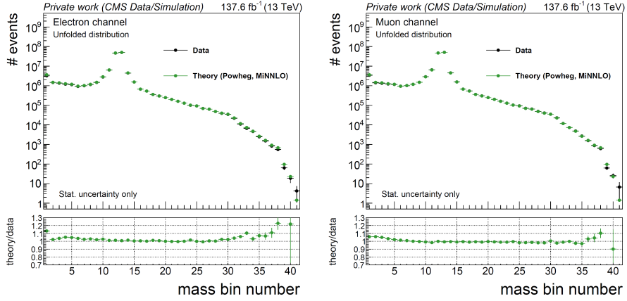
Fig. 43: Comparison of unfolded data with the generator-level prediction from the nominal signal simulation for electrons (left) and muons (right), with all data-taking eras combined.
