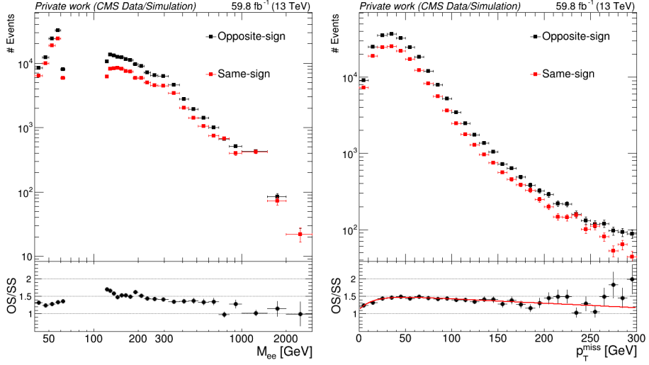
Fig. 35: Comparison of OS and SS dielectron invariant mass (left) and missing transverse momentum p_T^{\text{miss}} (right) distributions for misidentified/non-prompt electrons in the sideband where one electron fails the Medium ID requirement, for 2018 data. The red line shows the functional fit used to define the event weight in Eq. (10.10).
