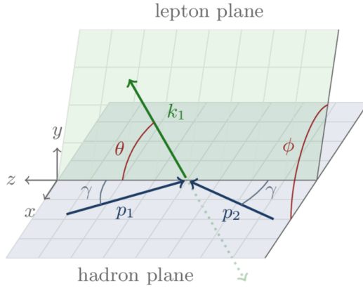
Fig. 8: An illustration of the Collins–Soper frame [61]. It is a dilepton center-of-mass frame, where k_1 and k_2 denote the lepton momenta and p_1 and p_2 denote the momenta of the incoming protons. The z -axis is chosen to bisect the angle between p_1 and -p_2 , while the x -axis is chosen to bisect the angle between p_1 and p_2 . The y -axis is perpendicular to the x – z plane. The polar angle \theta^* and azimuthal angle \phi^* describe the lepton orientation in this frame.
