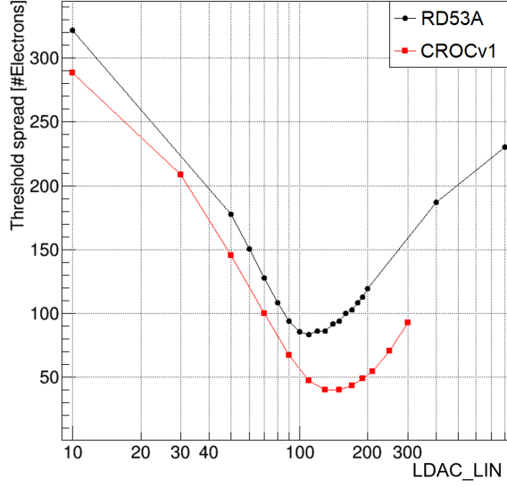
Fig. 60: Comparison of the threshold dispersion achieved with RD53A (black) and CROCv1 (red) chips at different LDAC values [A2, B2, B3].
