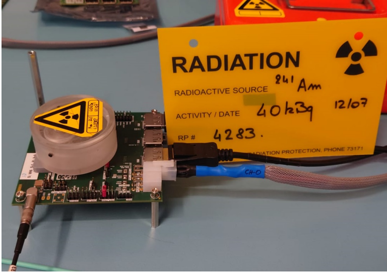
Fig. 65: A ^{241}\text{Am} source placed above the CROCv1 chip mounted on an SCC with a planar sensor during the X-ray calibration measurement.
