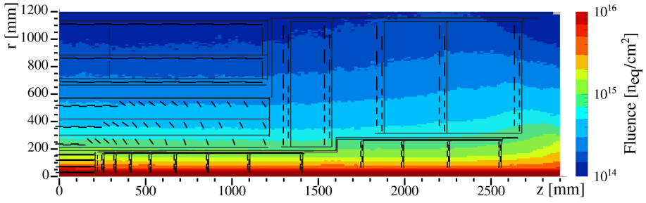
Fig. 48: Integrated particle fluence in 1 MeV neutron equivalent per \text{cm}^2 in the CMS Tracker for an integrated luminosity of 3000 \text{ fb}^{-1} at the HL-LHC [22]. The distance from the proton beam in the transverse direction is denoted by r , while the longitudinal distance from the collision point in the center of the CMS detector is shown by z [137].
