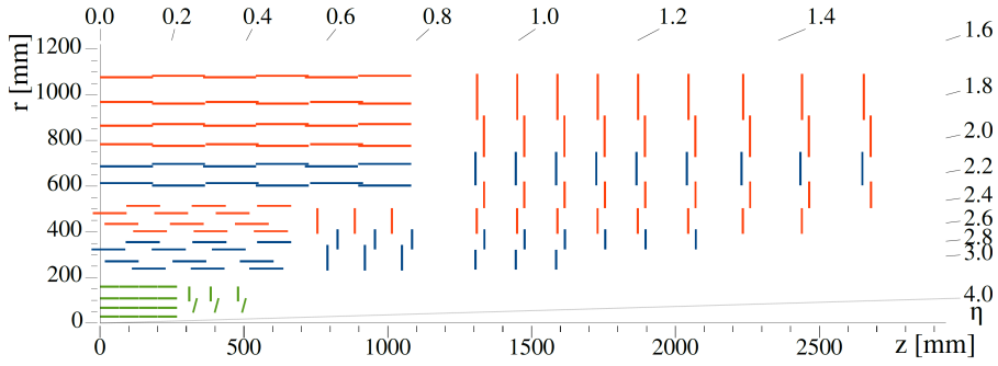
Fig. 49: A one-quarter slice of the current Phase-1 CMS Tracker in the r - z plane [137]. The silicon pixel detector modules are shown in green, while single-sided and double-sided silicon strip detector modules are shown in red and blue, respectively.
