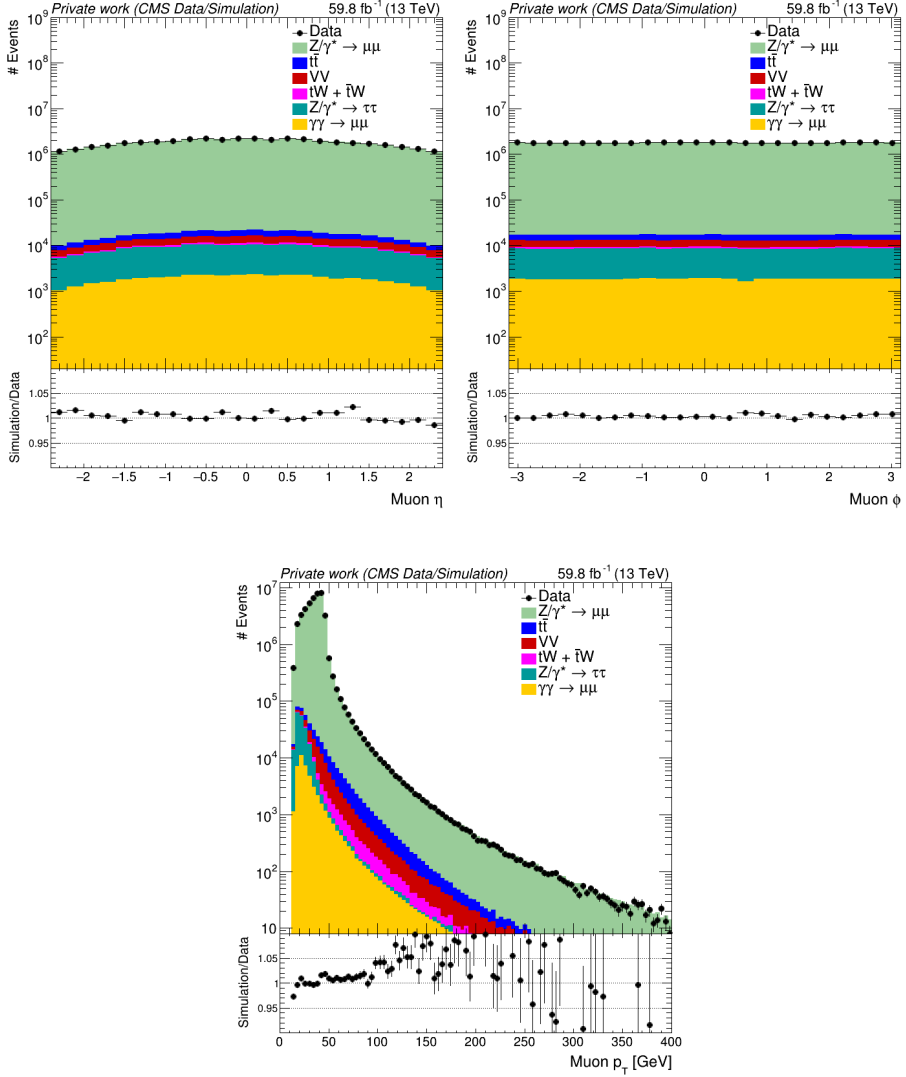
Fig. 17: Subleading-muon kinematic distributions for 2018 data and simulation after event selection and corrections.
