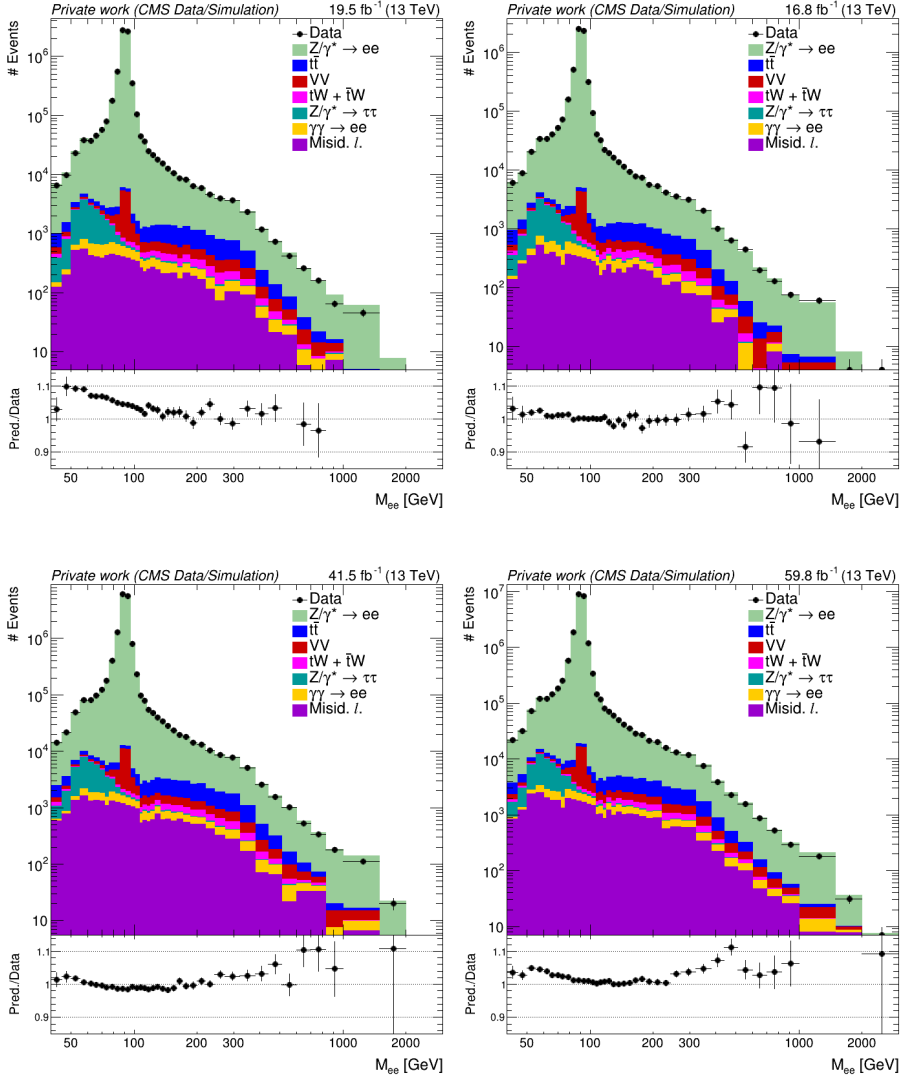
Fig. 40: Comparison between data and the total background prediction in the OS dielectron signal region after applying the e\mu -based top-quark reweighting and including the misidentified/non-prompt electron estimate, for each data-taking era: 2016 pre-APV (top left), 2016 post-APV (top right), 2017 (bottom left), and 2018 (bottom right).
