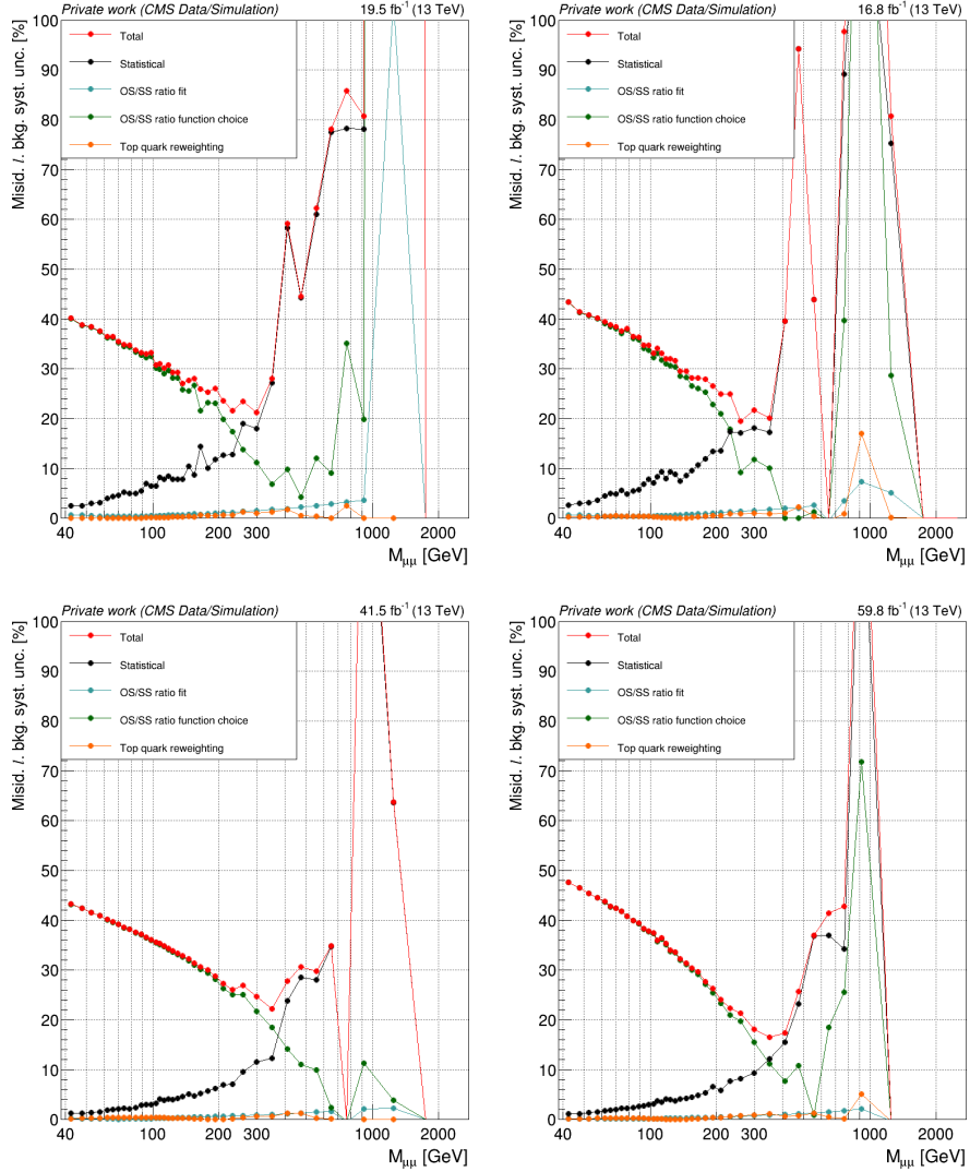
Fig. 27: Relative uncertainties on the misidentified/non-prompt muon background estimate for each data-taking era. Points with 0% uncertainty correspond to empty bins. Very large uncertainties at the highest masses are due to limited statistics in both the control and signal regions.
