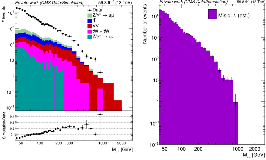
Fig. 22: Left: comparison between data and simulated prompt-lepton backgrounds in the SS dimuon control region for 2018 data. The excess of data over the sum of simulated distributions is attributed to events with misidentified/non-prompt muons. Right: estimated distribution of misidentified/non-prompt muons in the same region, obtained by subtracting the simulated prompt-lepton backgrounds from data.
