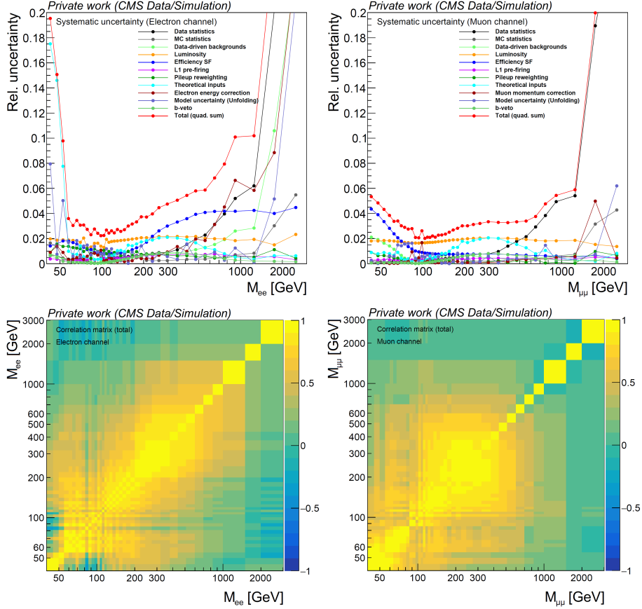
Fig. 44: Summary of the total relative uncertainties (top) and the total correlation matrices (bottom) for the electron (left) and muon (right) channels as a function of dilepton invariant mass.
