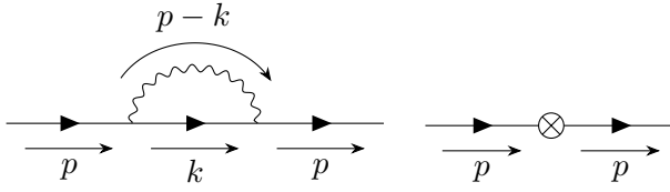
Fig. 4: One-loop electron self-energy diagram (left) and the corresponding counterterm diagram (right).
