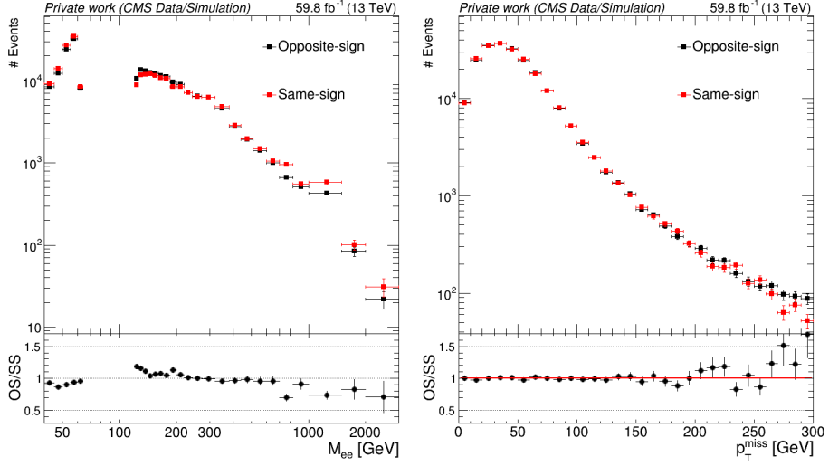
Fig. 36: Closure tests for the misidentified/non-prompt electron background in the sideband where one electron fails the Medium ID requirement. Shown are comparisons of OS data and reweighted SS data for the dielectron mass (left) and missing transverse momentum p_T^{\text{miss}} (right), for 2018 data.
