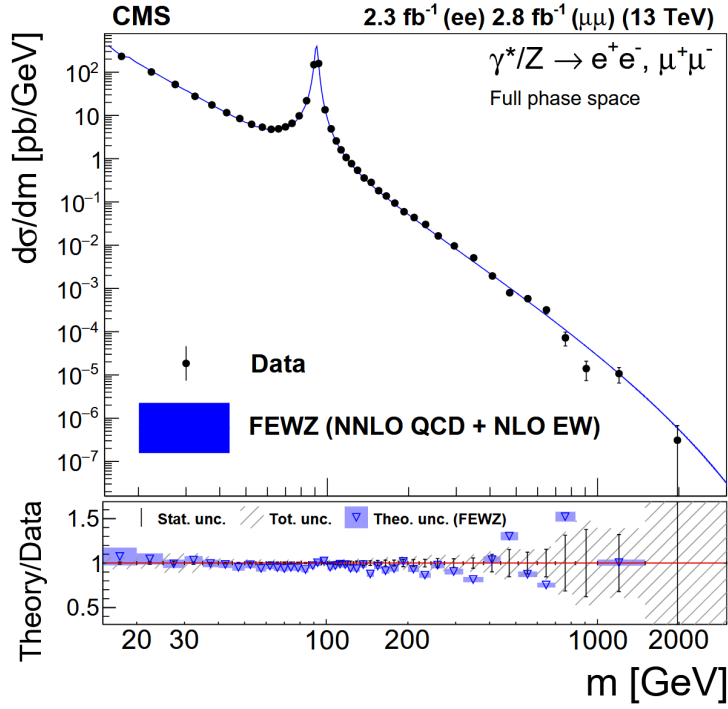
Fig. 10: The differential cross section d\sigma/dM of the Drell–Yan process measured by the CMS collaboration at \sqrt{s} = 13 TeV [19]. A comparison with the theoretical prediction calculated with FEWZ at NNLO in QCD and NLO in the electroweak theory is also shown.
