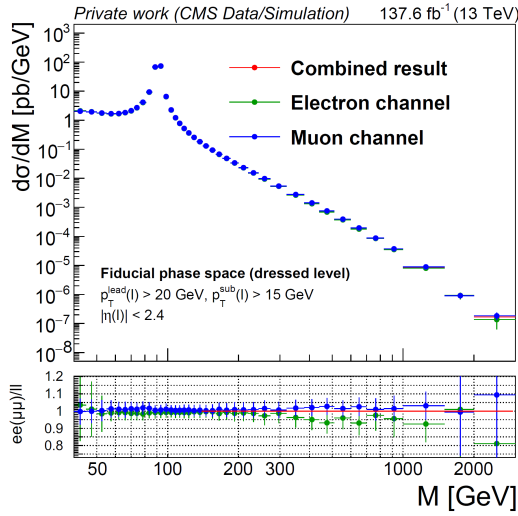
Fig. 45: Comparison between the combined and individual channel results for the measured Drell–Yan differential cross section.
