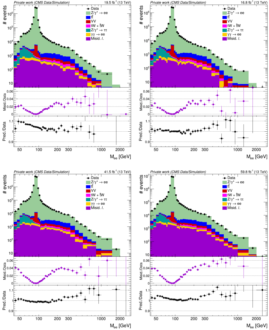
Fig. 39: Comparison between data and the sum of simulated prompt-lepton backgrounds plus the misidentified/non-prompt electron estimate in the OS dielectron signal region for each data-taking era. The middle panel shows the fraction of the observed data attributed to misidentified/non-prompt electron backgrounds, while the bottom panel shows the ratio of the total signal plus background prediction and the observed data.
