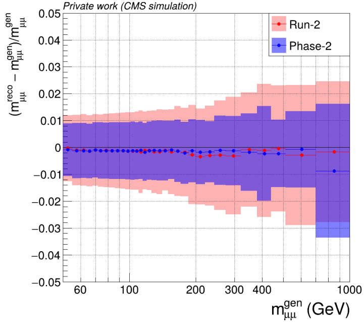
Fig. 70: Comparison of the reconstructed-to-generator response for the dimuon invariant mass in Run-2 and Phase-2 as a function of the generator-level M_{\mu\mu} . In each generator-level bin, the response distribution is fitted with a Gaussian function. The marker points show the fitted mean, while the shaded bands indicate the fitted width \sigma , taken as the resolution.
