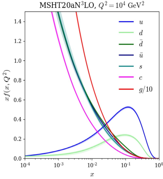
Fig. 5: Examples of parton distribution functions from the MSHT collaboration [43] at a factorization scale of 100 GeV. The PDFs are shown for different parton types, including quarks, antiquarks, and gluons.
