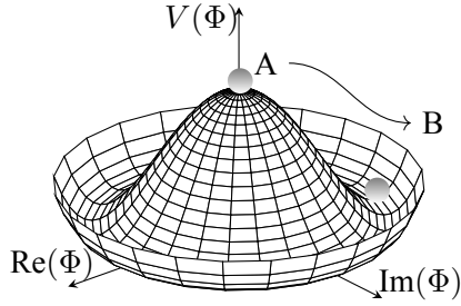
Fig. 2: The Higgs potential V(\Phi) as a function of the Higgs field \Phi for \mu^2 < 0 and \lambda > 0 . The circular groove at the bottom has a radius of v = \sqrt{-\mu^2/\lambda} and corresponds to the VEV.
