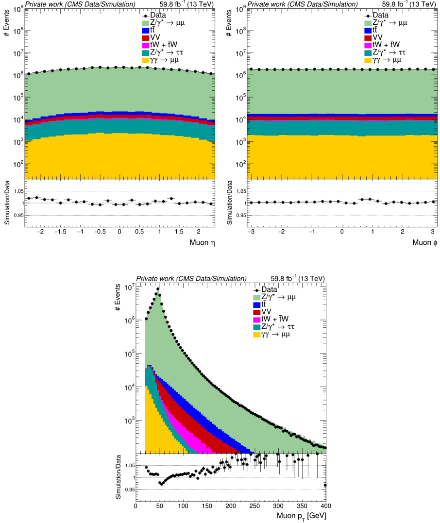
Fig. 16: Leading-muon kinematic distributions for 2018 data and simulation after event selection and corrections.
