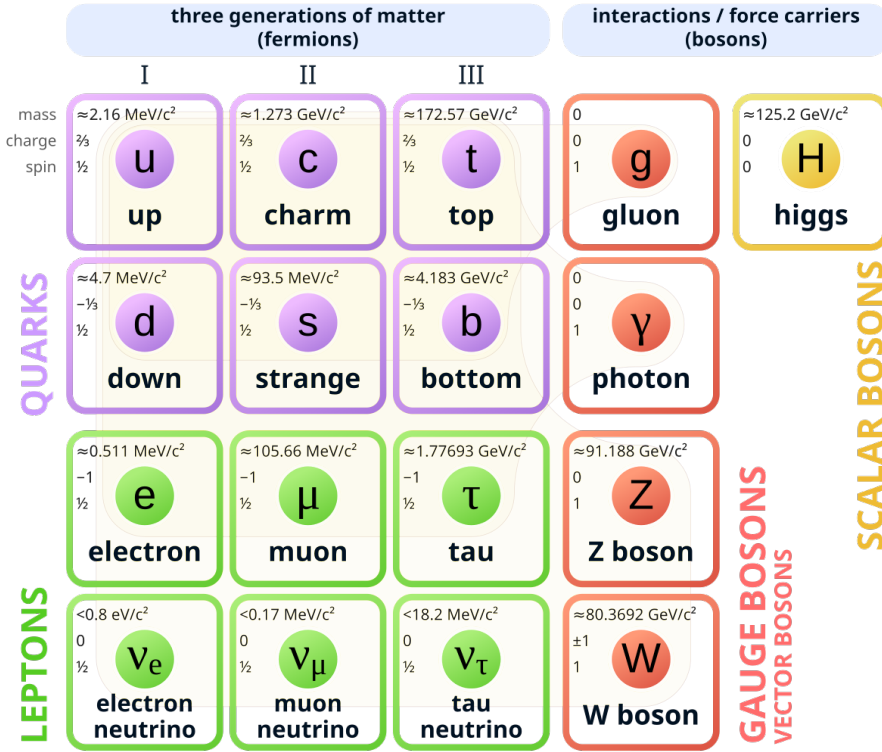
Fig. 1: The fundamental particles in the Standard Model, divided into fermions and bosons. Each of the first three columns represents a generation of fermions, while the second column from the right lists the gauge bosons that mediate the fundamental interactions. The rightmost column contains the Higgs boson [39].
