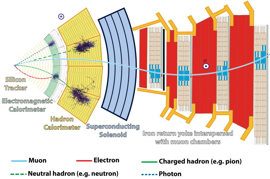
Fig. 13: A cross-sectional slice of the CMS detector [107].
