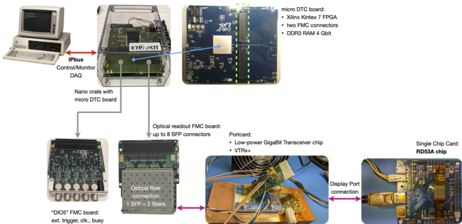
Fig. 53: Main components of the module testing and characterization setup. Adapted from Ref. [159].
