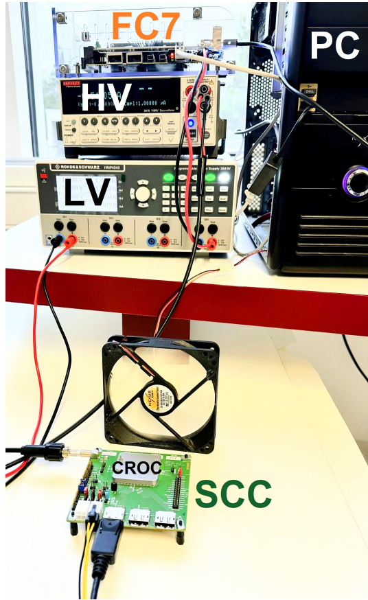
Fig. 58: Test setup used for prototype testing at Vilnius University. “FC7” denotes the back-end board, “PC” the Linux computer, “HV” the high-voltage power supply, “LV” the low-voltage power supply, “SCC” the Single-Chip Card, and “CROC” the CROCV1 readout chip mounted on the SCC.
