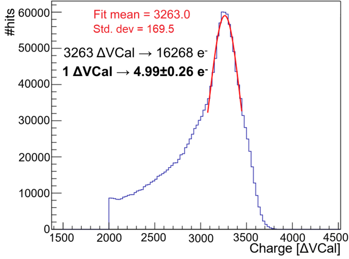
Fig. 67: Signal distribution of the recorded ^{241}\text{Am} X-ray hits. Only single-pixel clusters are considered. The signal is measured in \Delta\text{VCal} units [B3].
