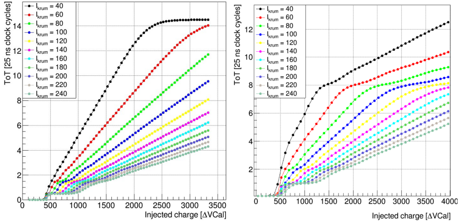
Fig. 63: Average ToT response as a function of injected charge for different Krummenacher current settings. Left: without 6-to-4-bit compression; right: with 6-to-4-bit compression enabled. The hit-detection threshold is fixed to approximately 2000 electrons [B3].
