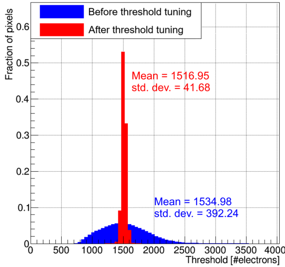
Fig. 59: Threshold distribution of a tested CROCv1 chip before (blue) and after (red) TDAC tuning at an average threshold of approximately 1500 electrons [B3].
