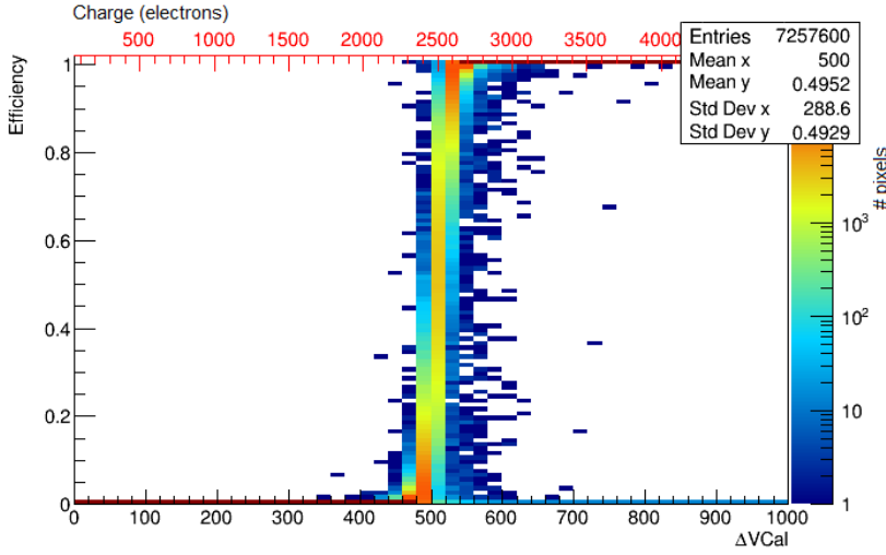
Fig. 56: Example of superimposed S-curves for all pixels on a chip, produced by the S-curve scan.
