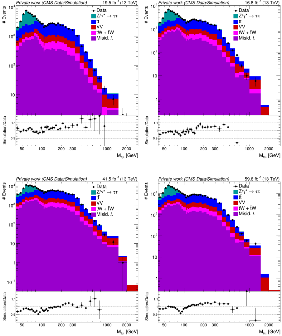
Fig. 30: Comparison between data and the sum of simulated backgrounds plus the misidentified/non-prompt lepton estimate in the OS e\mu control region for each era. A systematic overestimate of the total background at high invariant mass is visible.
