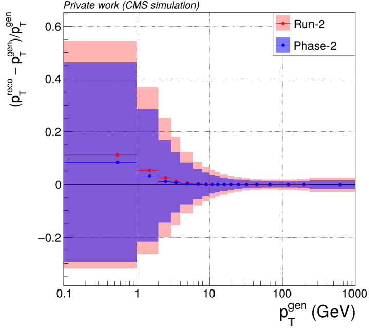
Fig. 71: Comparison of the reconstructed-to-generator response for the dimuon transverse momentum in Run-2 and Phase-2 as a function of the generator-level p_T^{\mu\mu} . In each generator-level bin, the response distribution is fitted with a Gaussian function. The marker points show the fitted mean, while the shaded bands indicate the fitted width \sigma , taken as the resolution.
