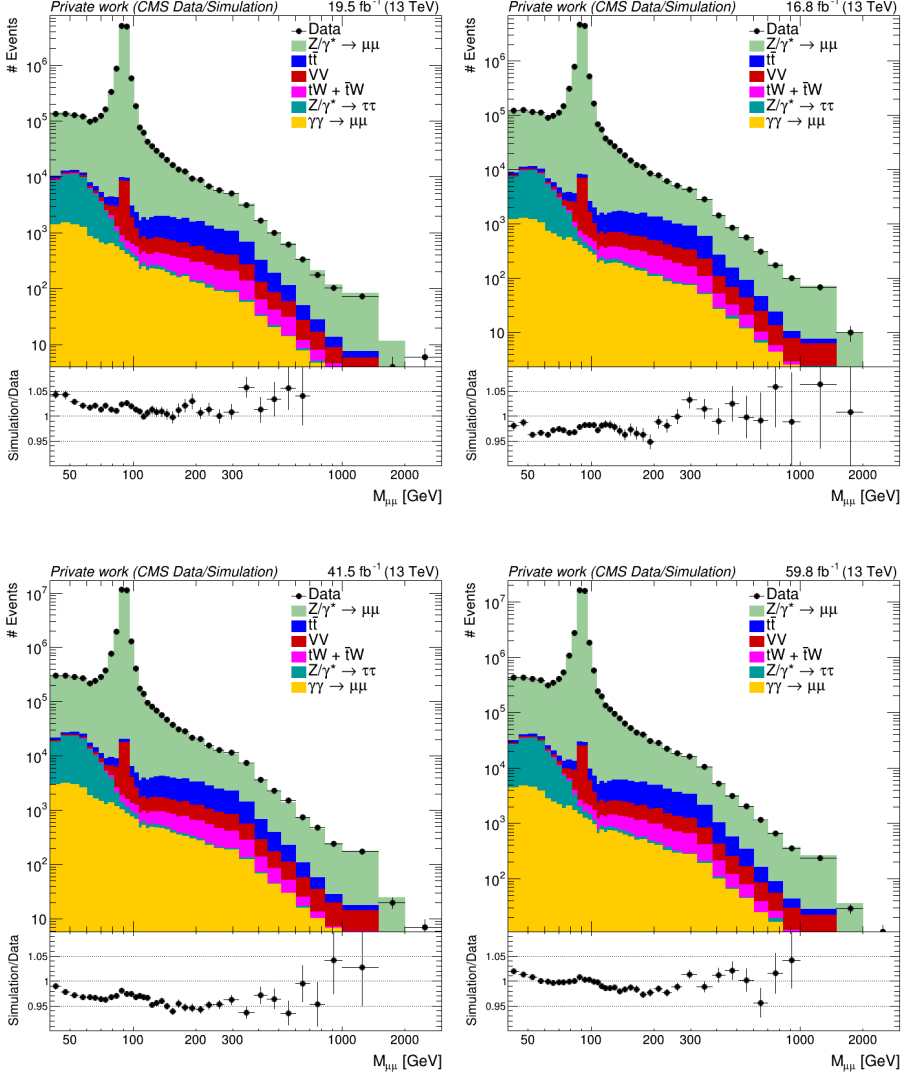
Fig. 18: Dimuon invariant mass distributions for all eras after event selection and corrections.
