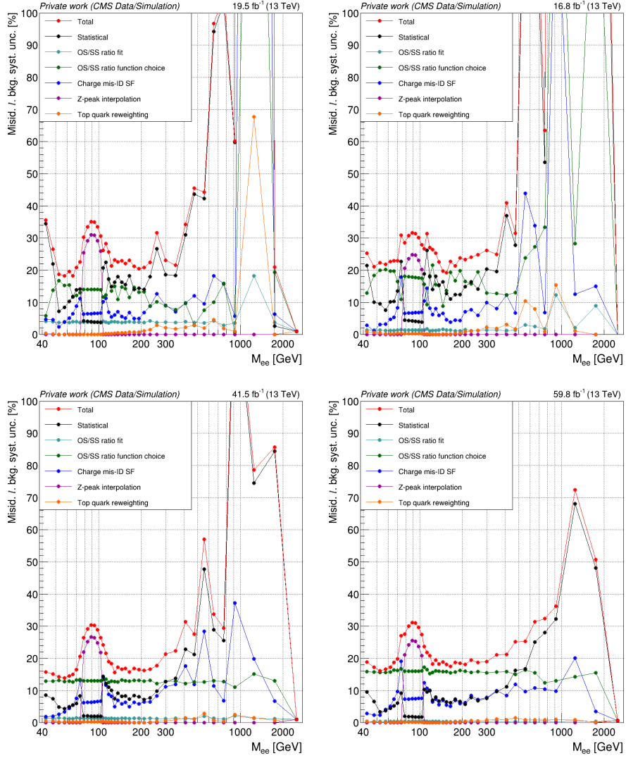
Fig. 38: Relative uncertainties on the misidentified/non-prompt electron background estimate for each data-taking era. Points with 0% uncertainty correspond to empty bins. Large uncertainties at the highest masses arise from limited statistics in the control and signal regions.
