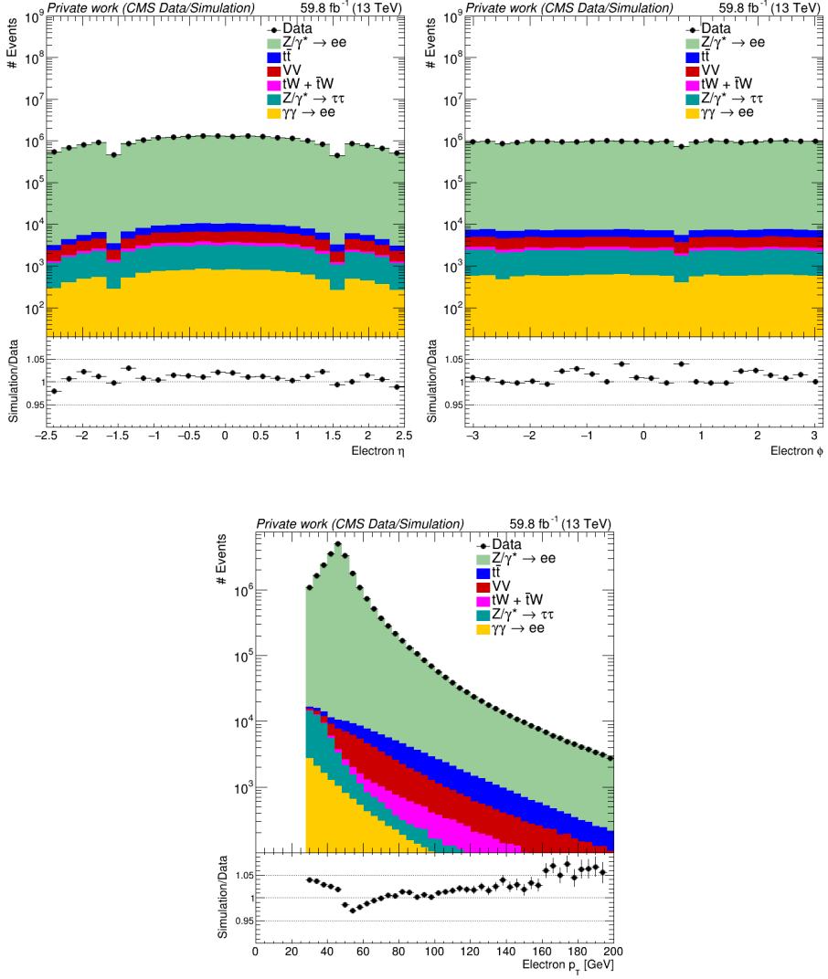
Fig. 19: Leading-electron kinematic distributions for 2018 data and simulation after event selection and corrections.
