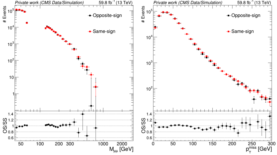
Fig. 25: Closure tests for the misidentified/non-prompt muon background estimate in the data sideband. Shown are the dimuon mass (left) and missing transverse momentum p_T^{\text{miss}} (right) distributions for OS data and reweighted SS data for 2018.
