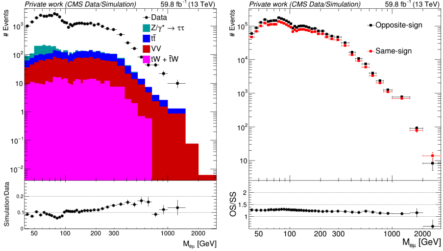
Fig. 29: Left: comparison of data and simulated prompt-lepton backgrounds in the SS e\mu sample. The excess of data is attributed to misidentified/non-prompt leptons. Right: comparison of OS and SS e\mu invariant mass distributions in the sideband where the electron fails the Medium ID requirement. The approximate flatness of the ratio motivates the use of a constant OS/SS transfer factor, R_{\text{OS/SS}} = 1.27 , in the e\mu channel. Both plots are shown for 2018 data; the other eras exhibit similar behavior.
