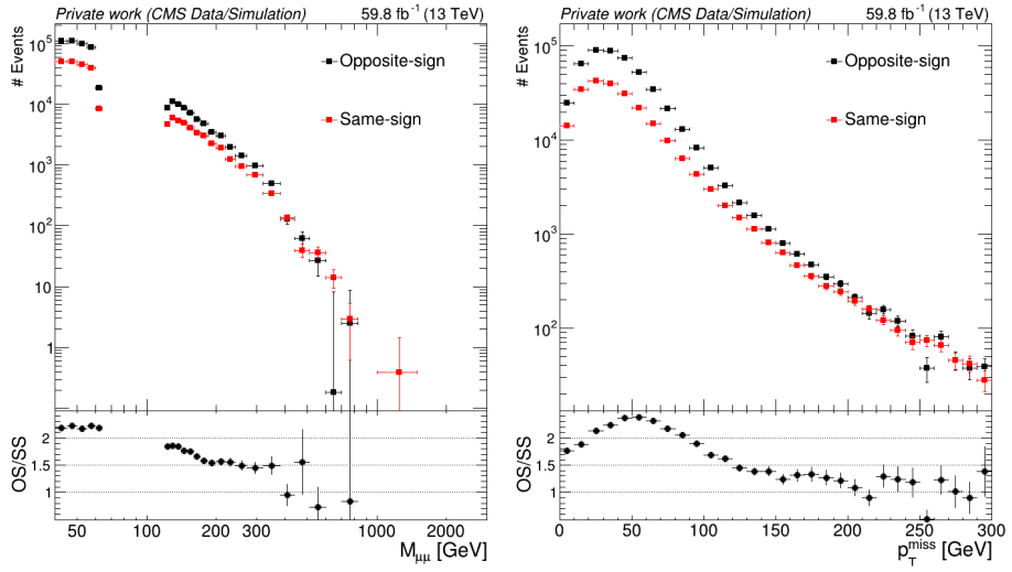
Fig. 23: Comparison of OS and SS dimuon invariant mass (left) and missing transverse momentum p_T^{\text{miss}} (right) distributions for misidentified/non-prompt muons in the data sideband where exactly one muon fails the isolation requirement. The distributions are shown for 2018 data; the other eras show similar behavior.
