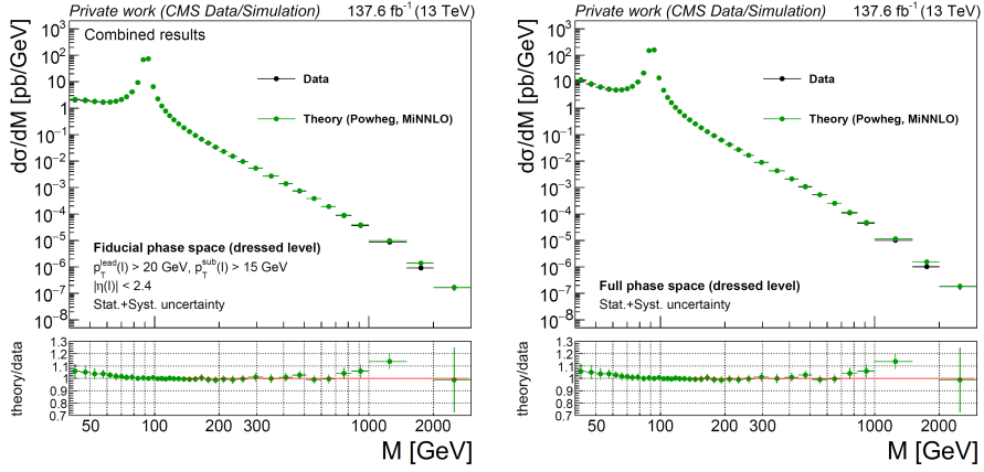
Fig. 46: Comparison of the combined Drell–Yan differential cross section with the SM prediction from POWHEG MiNNLO in the fiducial phase space (left) and extrapolated to the full phase space (right).
