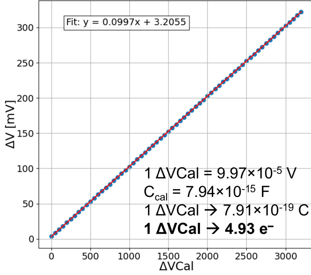
Fig. 64: Calibration voltage measured through the voltage multiplexer as a function of \Delta V_{\text{Cal}} [B3].
